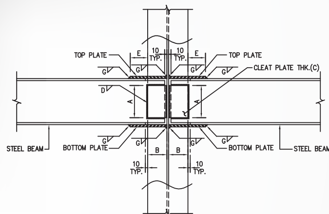
ELEVATION TYPE "B"
